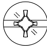
COMBO ACR® PHILLIPS II®
