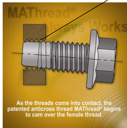
Threads Cam Into Alignment
