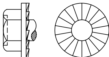
SERRATIONS
