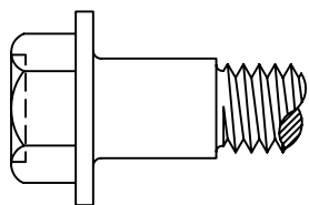
SHOULDER
