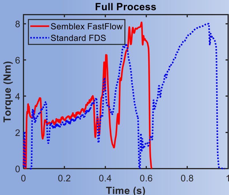
Data for 2mm on 2mm 6061-T6 Aluminum stackup on DEPRAG Adaptive DFS
