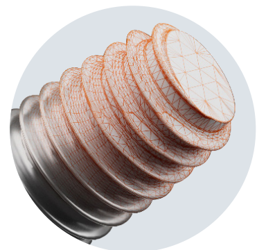
Progressive Forming Profile at the tip of the ALtracs® Xt
