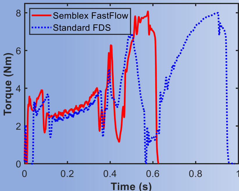
Data for 2mm on 2mm 6061-T6 Aluminum stackup on DEPRAG Adaptive DFS
