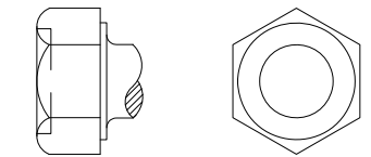
Washer Face
